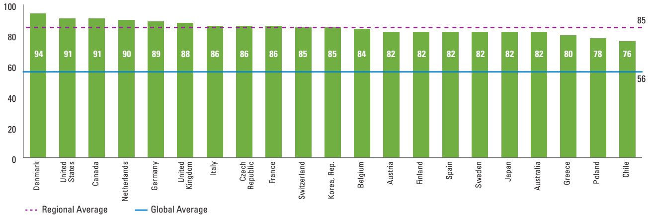
FIGURE 1 Overall Scores
